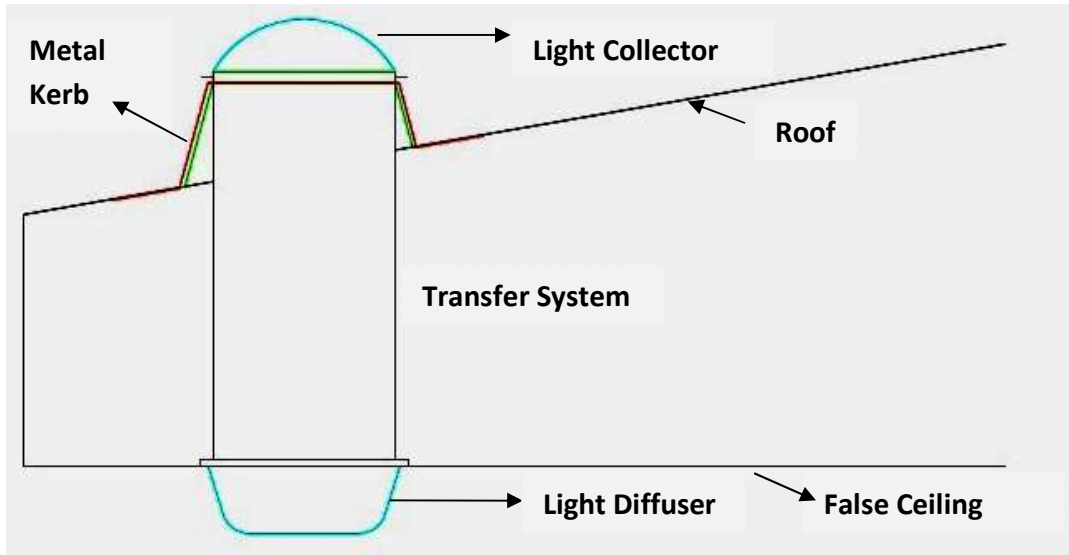
Fig.1 General Arrangement
